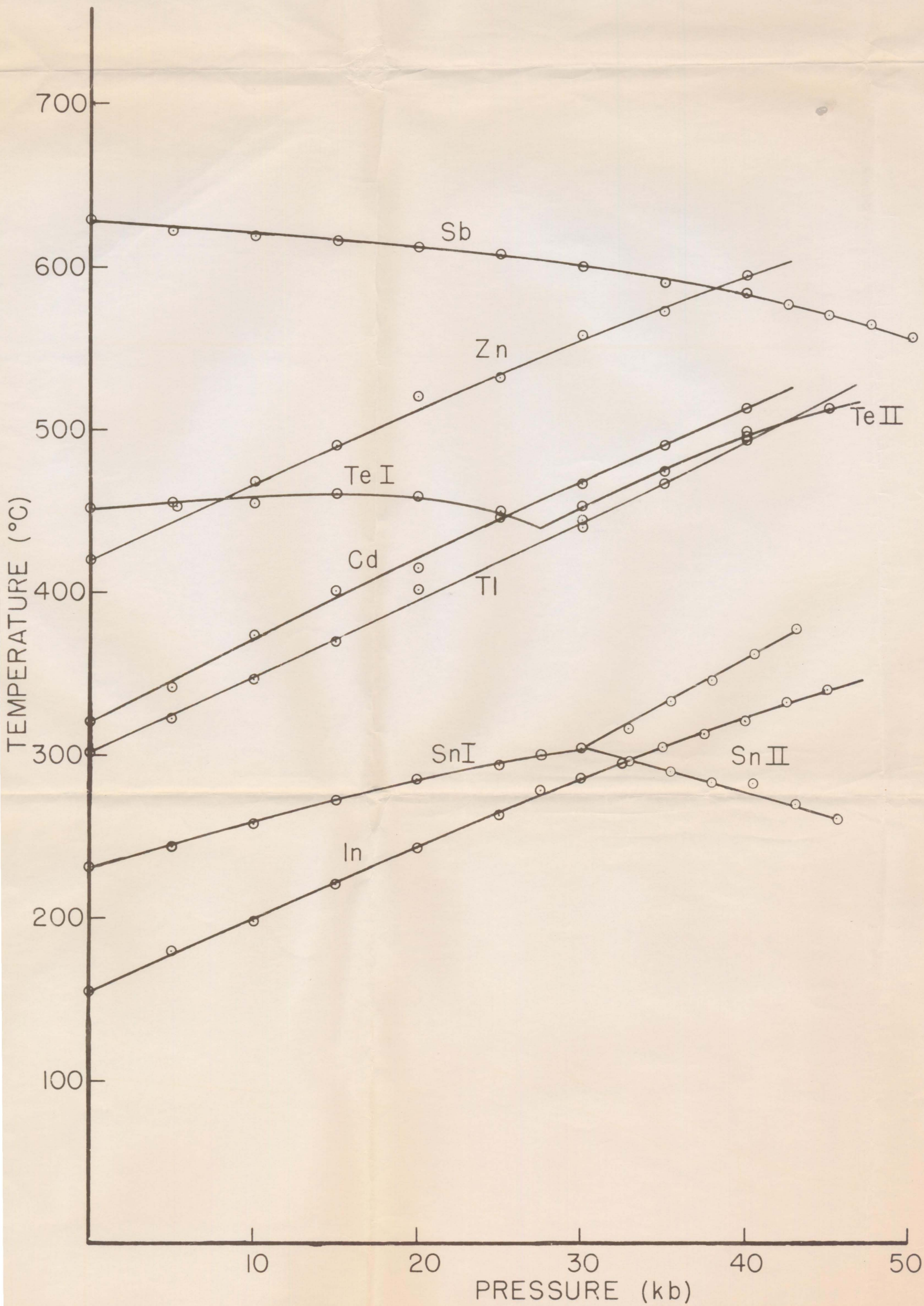
MELTING POINTS AT HIGH PRESSURES OF SEVEN METALS
